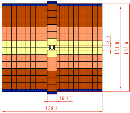
Fig. 2. The layout of one layer in the TT-station (TTb) is shown. The entire LHCb angular coverage is provided by silicon strip detectors. Short ladders are used in the centre along the bending plane where the particle densities are highest.
