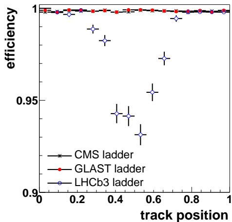
Fig. 7. Comparison of the cluster finding efficiency depending on the relative positions of the incident particle w.r.t. the readout strips for the different ladders.
