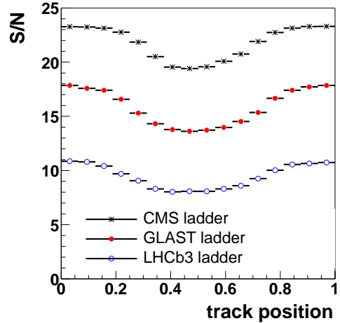
Fig. 6. Comparison of the S/N depending on the relative positions of the incident particle w.r.t. the readout strips for ladders with different sensor thickness.
