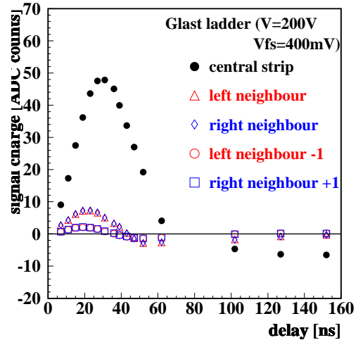
Fig. 3. Pulse shape on the central strips, their neighbours and their next neighbours.
