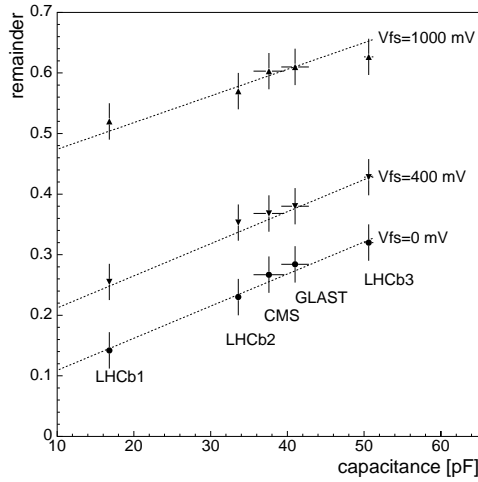
Fig. 4. Signal remainder after 25 ns, i.e. one bunch crossing.
