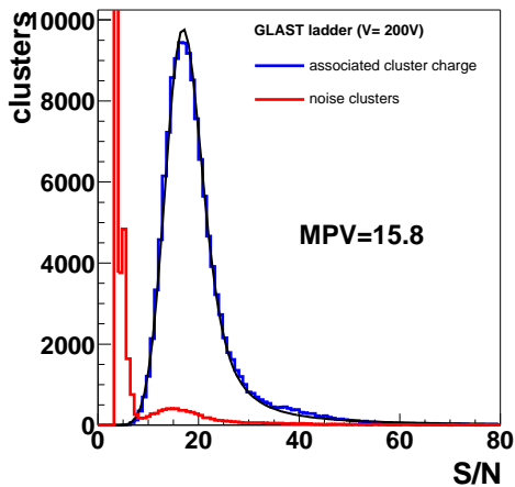
Fig. 5. S/N averaged over the positions of the particles relative to the readout strips.
